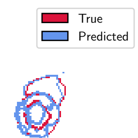
segmentations
